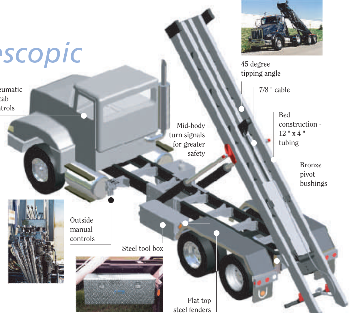
Frame mounted hydraulic tank - for greater accessibility
